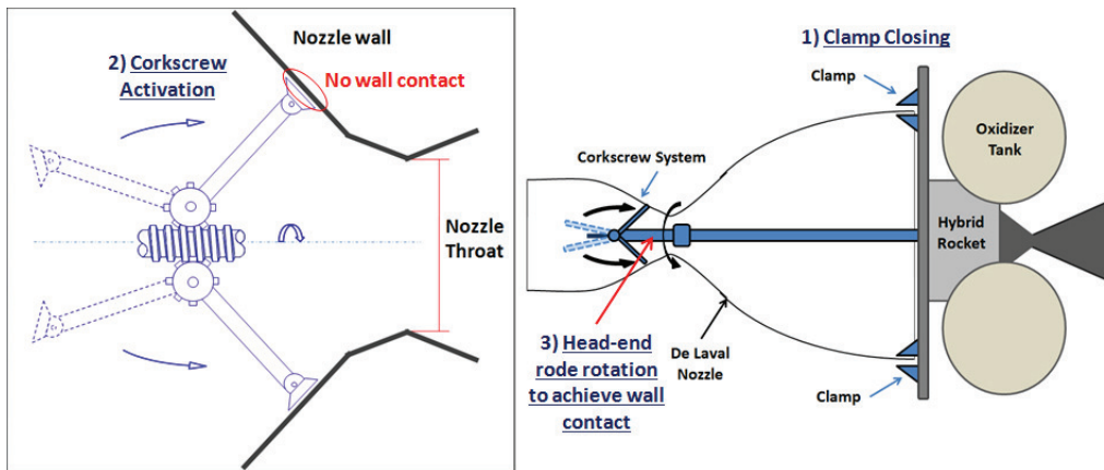
Figure 9: Corkscrew system mechanism.
